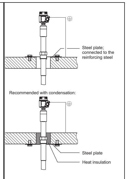
Silo with concrete walls
